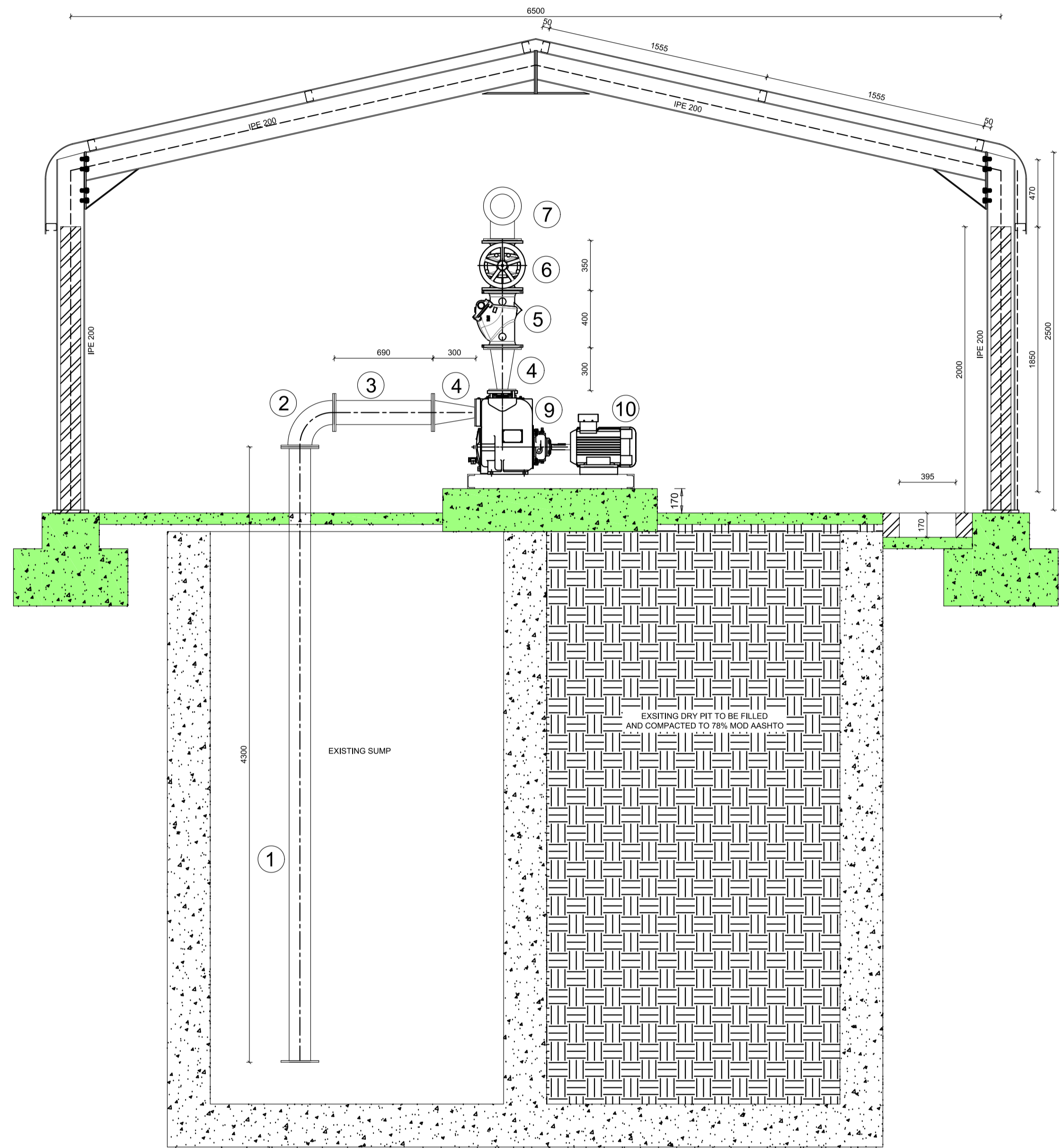
ROOF STRUCTURE SECTION SCALE 1:20
